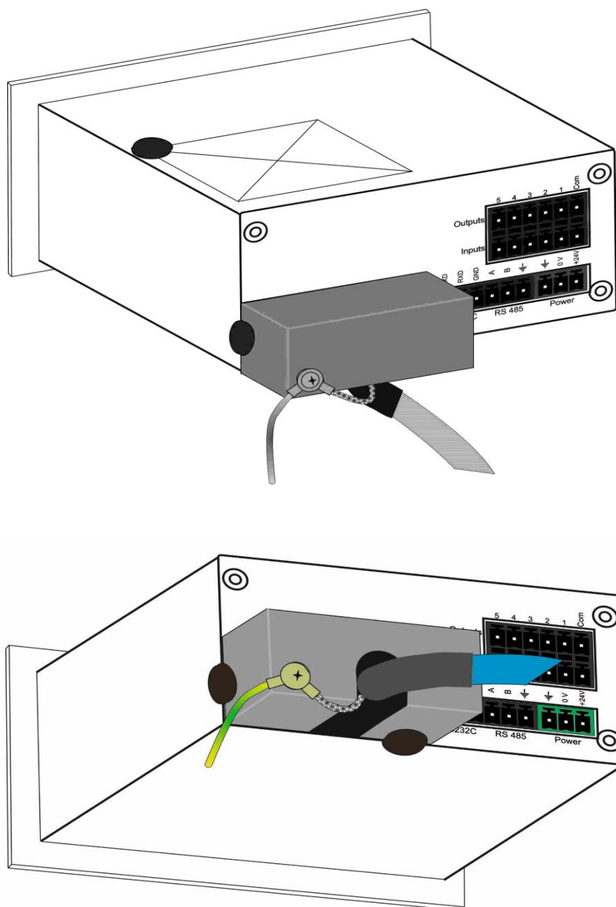
Figure 3 Sealing of FT-10 / FT-10 Fill / FT-10 Flow indicator with brittle stickers.
